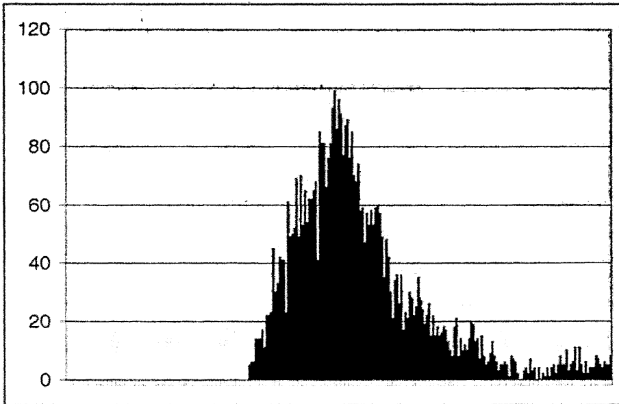
Figure 12. - Empirical distribution of Q_\lambda(\alpha, \beta^*) : 2 distinct tree shapes on 14 objets, 5 000 independent random permutations.
