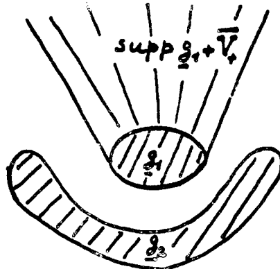
Fig. 1 \text{Supp. } g_1 \supset \text{Supp. } g_2
