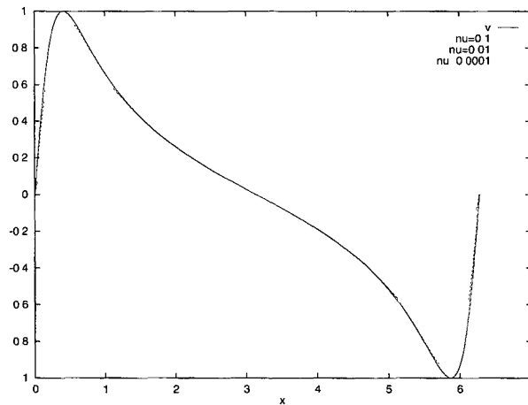
FIGURE 2 Convergence of the two-level method.
