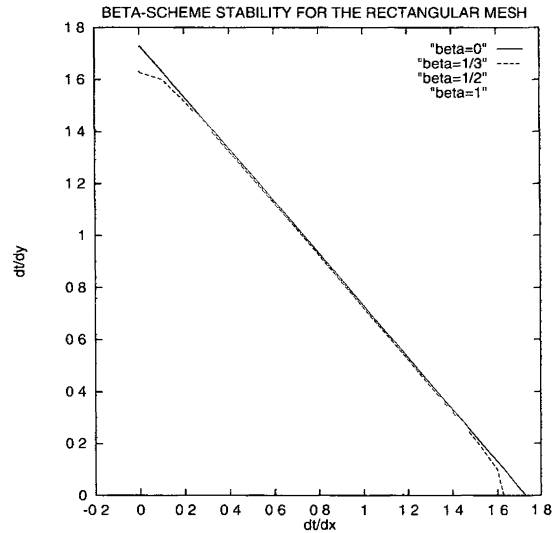
FIGURE 7. Convection equation.
