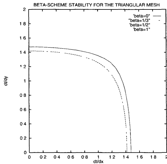
FIGURE 8. Maxwell system.
