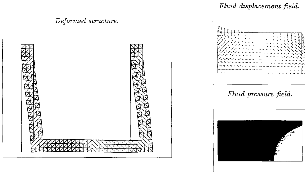
FIGURE 4. Hydroelastic vibration mode of frequency \omega_1^H .
