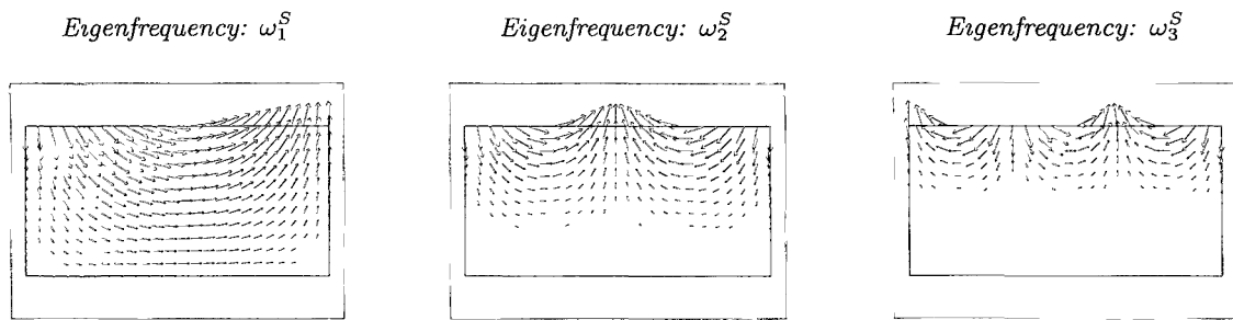
FIGURE 3. Fluid displacement fields of the lowest frequency sloshing modes.
