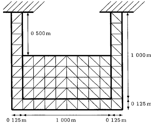
FIGURE 2. Steel vessel filled with water: geometrical data and initial mesh.
