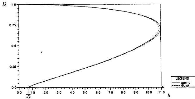
Figure 8. — Comparison of f_0^c(h) for the GL equations and the approximate model when \kappa = 0.003 .
