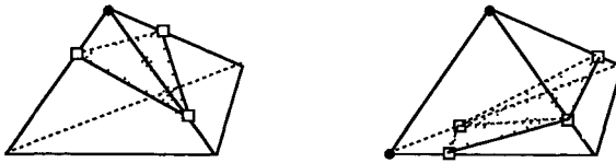
Figure 3. — Contour triangles in a tetrahedron.
