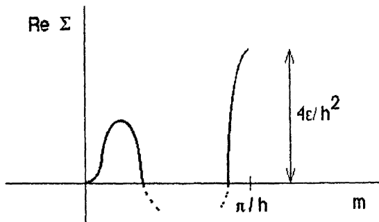
Figure 2. — Symbol of the space discretization (2.3).
