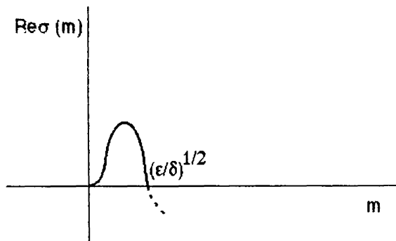
Figure 1. — Partial differential equation symbol.
