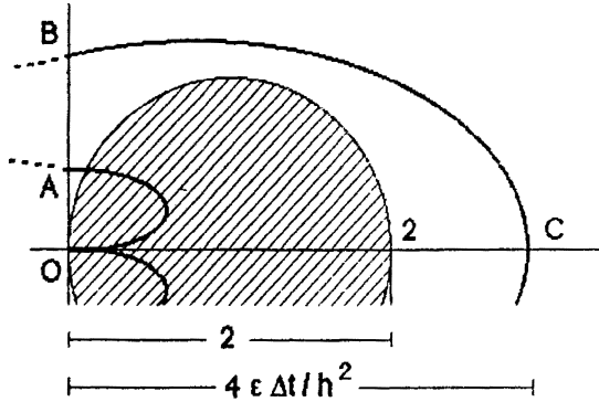
Figure 3. — Instability region of the Backward Euler method and schematic plot of locus \Delta t \Sigma(m, h) , with \Sigma(m, h) an eigenvalue of the system of ordinary differential equations (2.3) being integrated in time.
