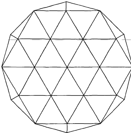
Figure 3. — 25 nodes \left( h = \frac{\sqrt{6} - \sqrt{2}}{2} \right) .
