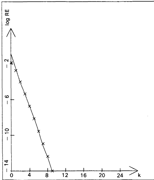
Figure 2. — Fredholm's Approximation n = 5 M = 101
