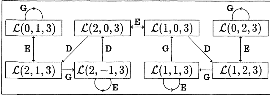
FIGURE 3. Graphe \zeta(3)
