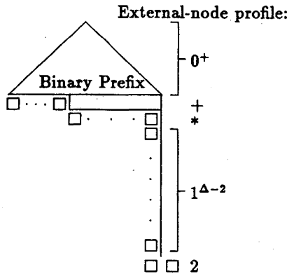
Figure 6. – A right-weighted (a, \Delta, N) -tree, where a = -1 .
