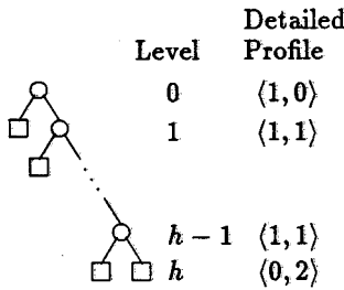
Figure 5. - A snake of height h . A Snake(h) has size h and its external path length is h \cdot (h+3)/2 .
