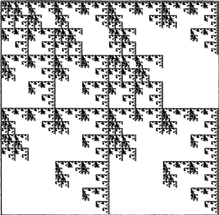
Adjacency Matrix
