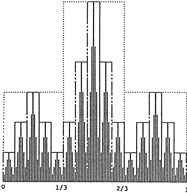
Fig. 1. A prototype of the hairy arc \mathbb{H} .
