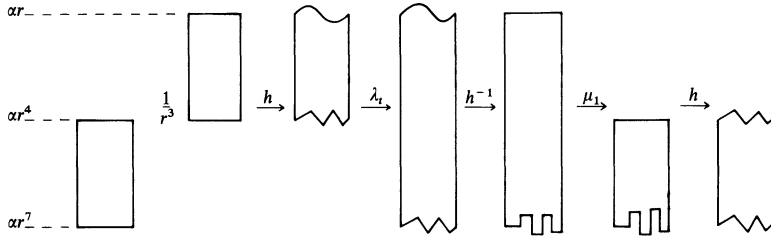
Figure 1. Definition of h_1 on c_{\alpha r^4}X - c_{\alpha r^7}X
