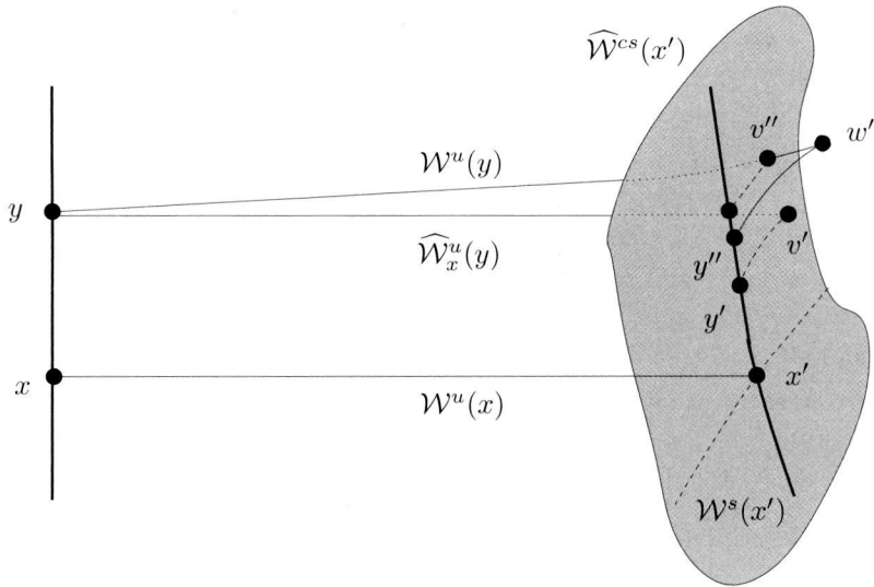
FIGURE 7. Points in the proof of Lemma 10.9
