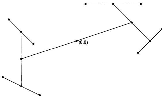
Figure 1: A martingale in the plane
