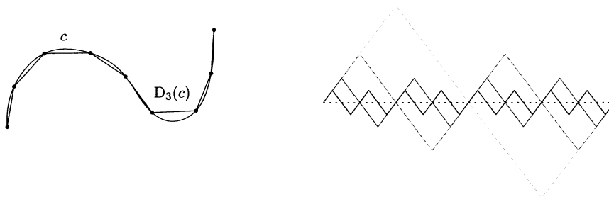
FIGURE 4. Left: a piecewise geodesic approximation of a path. Right: a Cauchy sequence for d_\ell which does not converge to its uniform limit, the dotted straight line.
