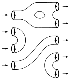
FIGURE 2. A surface seen as a topological transition between two collections of circles
