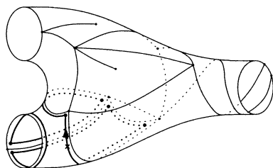
FIGURE 9. A possible track followed by our explorer. The landing point is denoted by a cross.
