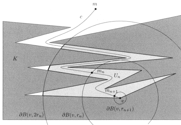
FIGURE 12. The path c_{n+1} will join m_n to m_{n+1} inside U_n .
