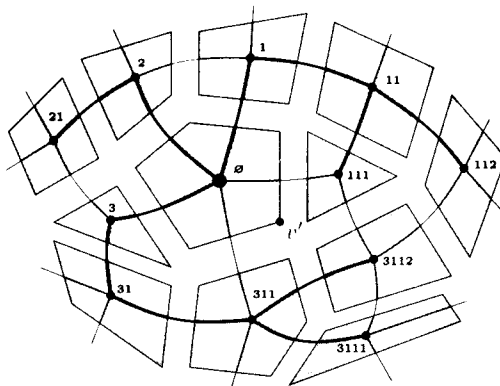
FIGURE 3. The labelling of the faces of a graph by words of integers. The vertex v' determines the rooting of \widehat{T} .
