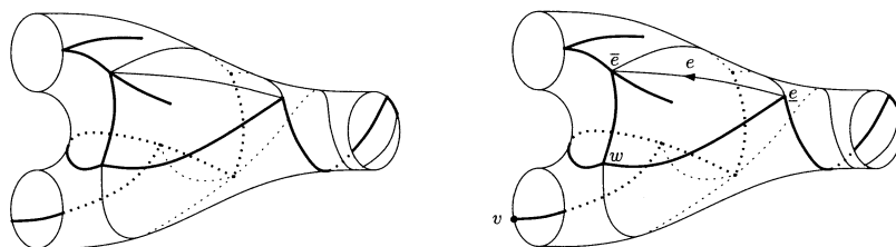
FIGURE 14. A spanning tree of our favourite graph. On the right, the position of the vertex w at which the injective paths [\underline{e}, v]_T and [\bar{e}, v]_T first meet, for a certain choice of v and e .
