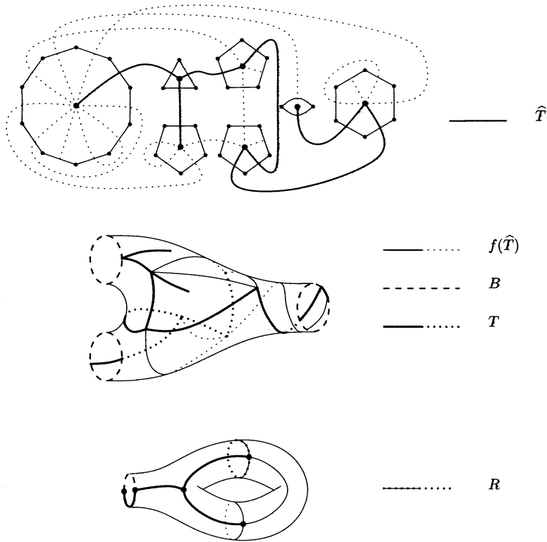
FIGURE 2. Two examples of partitions of the set of edges of a graph as R \cup B \cup f(\widehat{T}) \cup T . The first example is our favourite graph, and since it is a graph on a sphere, albeit with three holes, R is empty. In the much simpler second example, R contains one edge.
