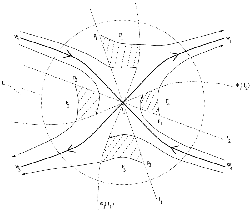
Fig. 5. How the fundamental domains are obtained.
