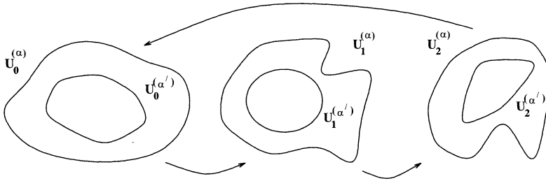
Fig. 3. D_\alpha \prec D_{\alpha'} with D_\alpha, D_{\alpha'} in a subchain of period three after suitable arrangement of indexes.
