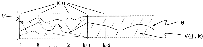
Fig. 2. Representation of the infinite product of the interval [0, 1] , a vector \underline{\theta} and the sets V and V(\underline{\theta}, k) .
