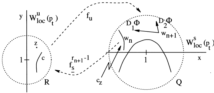
Fig. 7. The iterations in the proof of Proposition 11.2.
