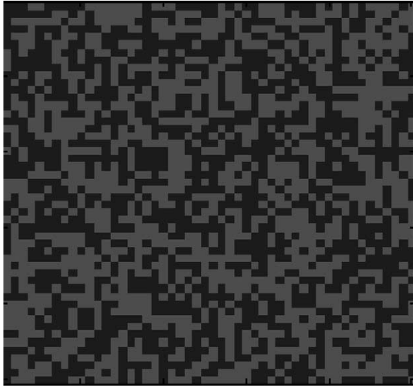
Fig. 1. Signs of the Gaussian field arising from the simple random walk on the 50 \times 50 discrete torus.
