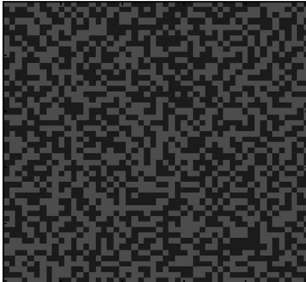
Fig. 2. Signs of the i.i.d. Gaussian field on the 50 \times 50 discrete torus.
