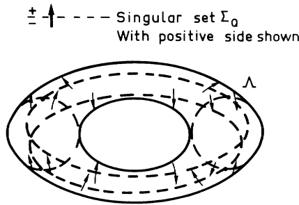
Fig. 4. — A typical l = 2 toric Lagrangian manifold.
