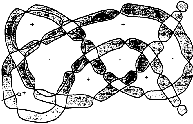
Fig. 7 Milnor fiber with vanishing cycles for y^4 - 2y^2x^3 + x^6 - x^7 - 4yx^5 .
