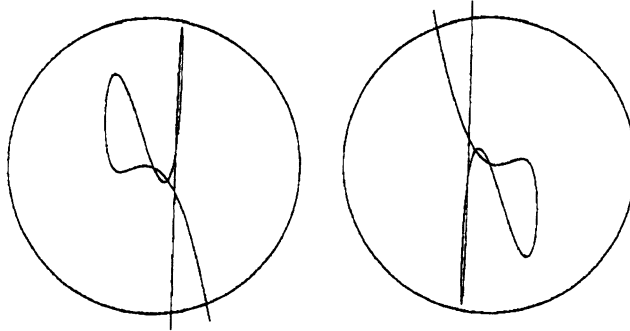
Fig. 2(a) The divides f_{\pm 1}(x, y) = 0 .
