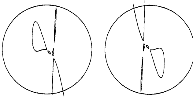
Fig. 2(b) Four ovals change parity.
