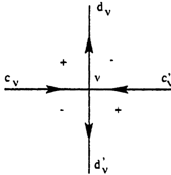
Fig. 3 The link P_v .
