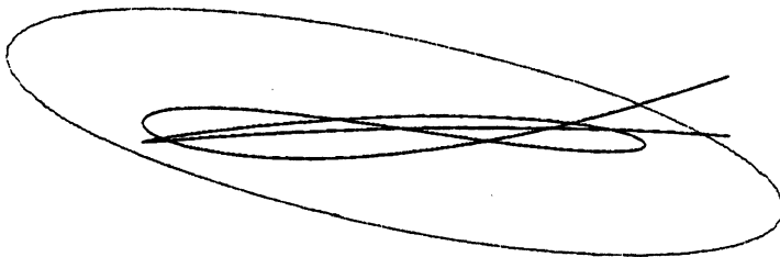
Fig. 9 The curve (x_s(t), y_s(t)) , s := 1 , as divide for the singularity of C .
