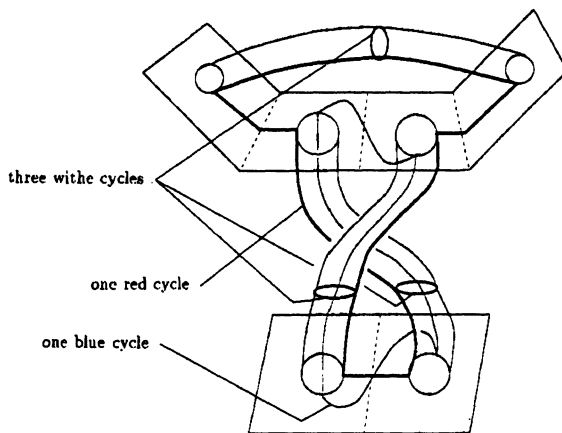
Fig. 6 Milnor fiber with vanishing cycles for D_5 .
