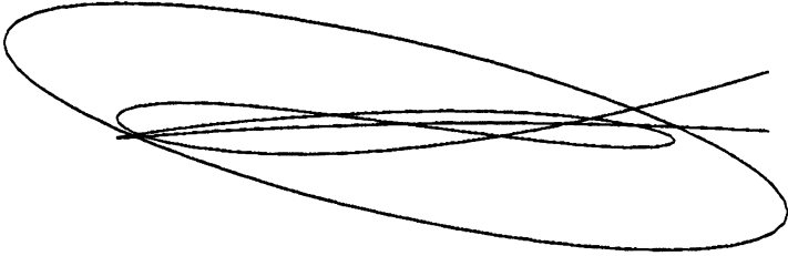
Fig. 11 A divide, which does not come from a singularity.
