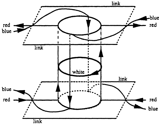
Fig. 4 A piece of surface F_v .
