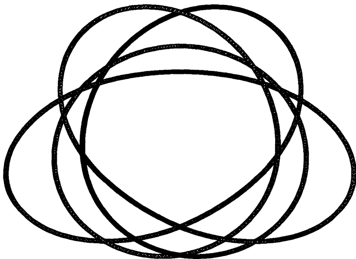
Fig. 8 The torus cable knot (2,3)(2,3) .
