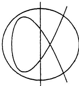
Fig. 5 A divide for the singularity D_5 .
