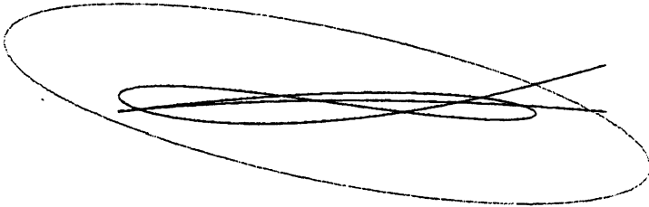
Fig. 10 The curves (x_s(t), y_s(t)) for s := 7\sqrt{2}/24 .
