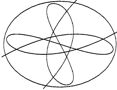
Fig. 1 A divide for (y^5 - x^3)(x^5 - y^3) = 0 .
