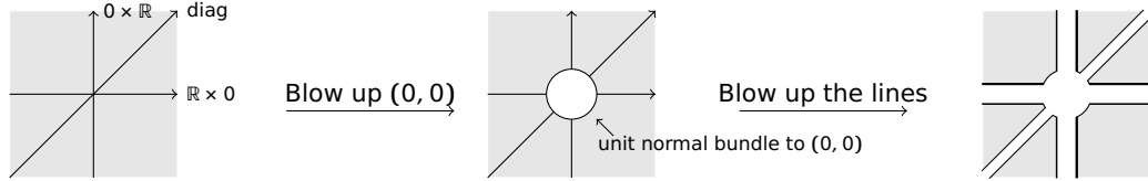
Figure 1.3: Iterated blow-ups of \mathbb{R}^2
