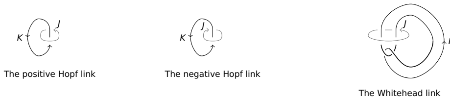
Figure 1.2: The Hopf links and the Whitehead link
