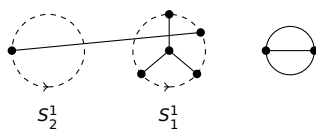
Figure 2.1: A Jacobi diagram \Gamma on the disjoint union \mathcal{L} = S^1_1 \sqcup S^1_2 of two (oriented) circles
