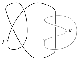
Figure 1.1: A 2-component link in \mathbb{R}^3
