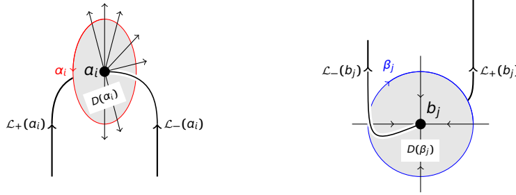
Figure 1.7: \mathcal{L}_+(a_i) , \mathcal{L}_-(a_i) , \mathcal{L}_+(b_j) , \mathcal{L}_-(b_j)
