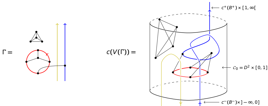
Figure 2.3: A (black) Jacobi diagram \Gamma on the source of an LTR L , and a configuration c of \check{C}(L; \Gamma)
