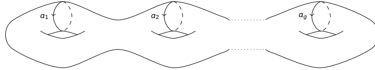
Figure 1.5: The standard handlebody H_g
