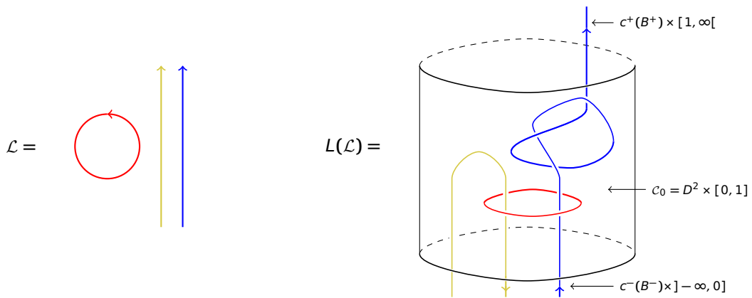
Figure 2.2: A long tangle representative (LTR) in \mathbb{R}^3
