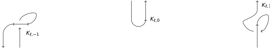
Figure 2.5: Long tangle representatives
