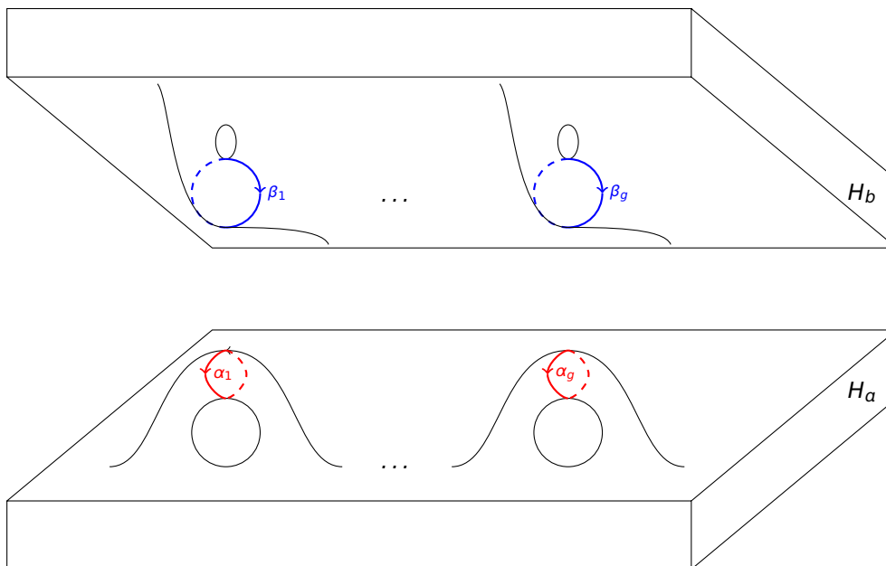
Figure 1.6: H_a and H_b
