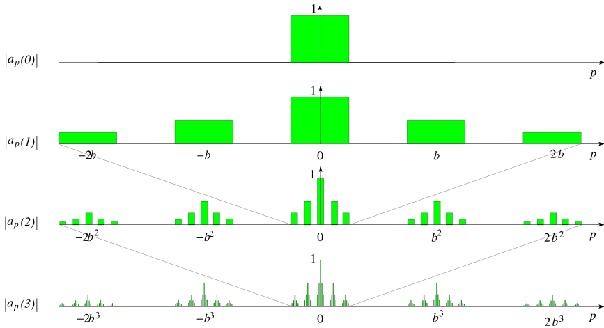
Figure 3.1. A schematic picture of the various spectra (a_p(k))_{p \in \mathbb{Z}} with N_k = b^k .
