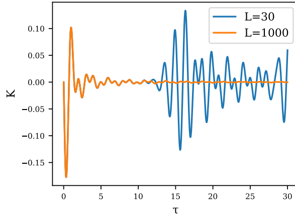
FIGURE 4.1. Time response function K_L(\tau) .
