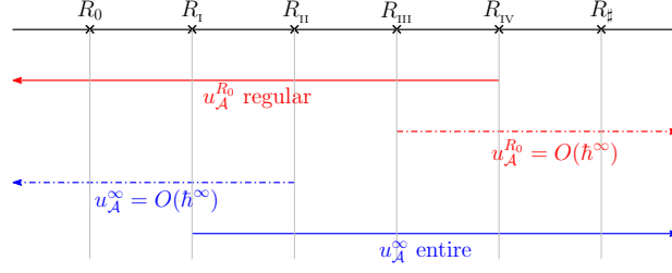
Figure 4.1: The splitting u_{\mathcal{A}} = u_{\mathcal{A}}^{R_0} + u_{\mathcal{A}}^\infty
