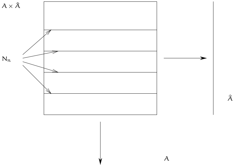
FIGURE 3.1. Factoring the universal cover of an abelian variety over k
