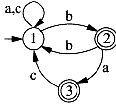
FIGURE 2. A trim minimal automaton.
