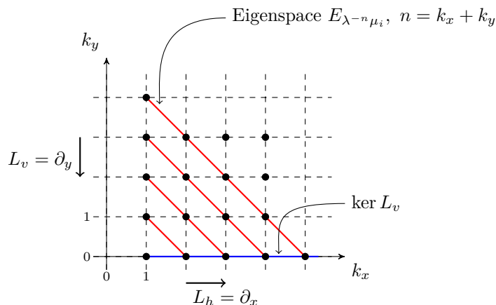
FIGURE 1.1. For a given eigenvalue \mu_i of T^* ( \mu_i \in (\lambda^{-1}, \lambda) ), each black point of the lattice (k_x, k_y)_{k_x \geq 1, k_y \geq 0} represents an independent Ruelle distribution u_{(k_x, k_y)} . In particular f_i = u_{(1,0)} . The eigenvalues of the transfer operator \mathcal{T} are \lambda^{-n} \mu_i with n \geq 1 and the associated eigenspace is E_{\lambda^{-n} \mu_i} = \text{Span} \{u_{k_x, k_y}, k_x + k_y = n\} with dimension n and represented by a diagonal red line. The operator L_h \equiv \partial_x maps u_{(k_x, k_y)} to u_{(k_x+1, k_y)} and L_v \equiv \partial_y maps u_{(k_x, k_y)} to u_{(k_x, k_y-1)} . In particular the space \ker L_v is represented by the first horizontal blue line k_y = 0 .
