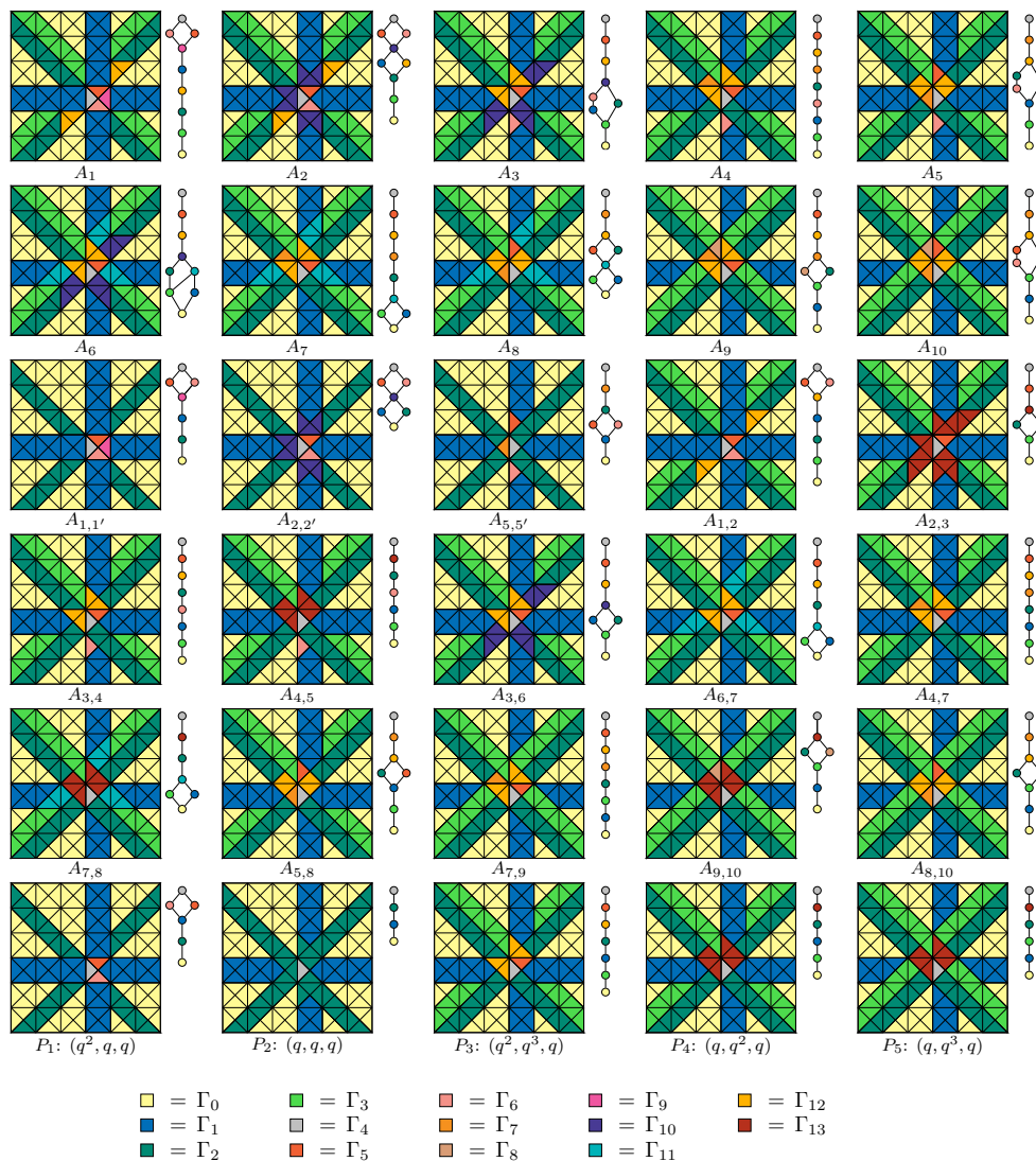
FIGURE 5. Decomposition of \tilde{C}_2 into cells for r_2 \leq r_1
