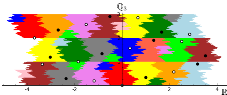
Figure 10.4. Tiling of the representation space K_\sigma with translation set \Gamma . The black (white) points belong to \Phi'(\text{Frac}(\sigma, 1)) (respectively \Phi'(\text{Frac}(\sigma, 2)) ).
