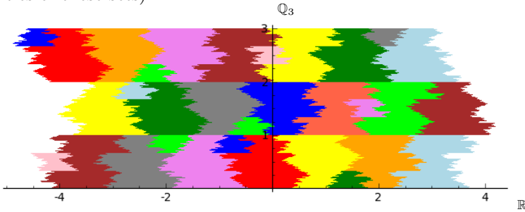
Figure 1.1. Tiling of the representation space K_\sigma associated with the 2-letter non-unit substitution \sigma(1) = 1^52, \sigma(2) = 1^3 .
