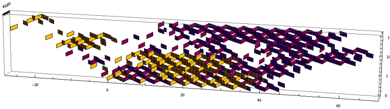
Figure 4.4. T_{\text{ext}}^{-4}((\mathbf{0}, 1) \cup (\mathbf{0}, 2)) for the substitution \sigma(1) = 2121^3 , \sigma(2) = 12 .
