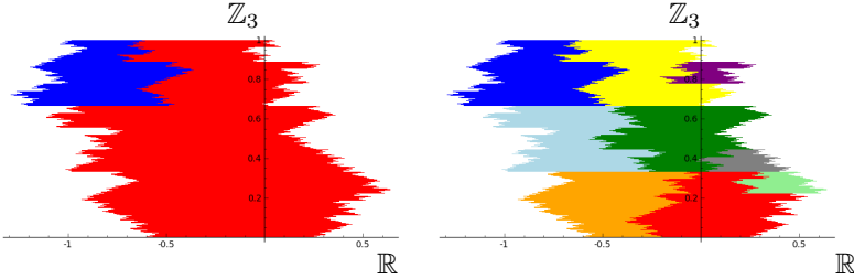
Figure 10.2. The central tile \mathcal{R}_\sigma divided in the red (light gray) subtile \mathcal{R}_\sigma(1) and the blue (dark gray) subtile \mathcal{R}_\sigma(2) , and the self similar structure arising from the set equations.
