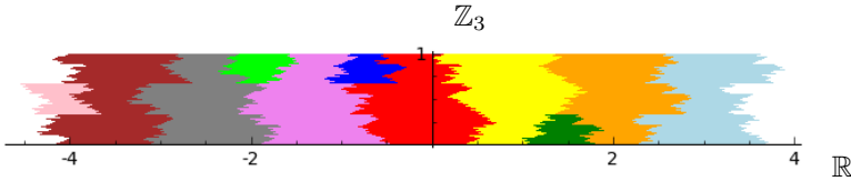
Figure 10.3. First 3-adic level of the tiling of K_\sigma .
