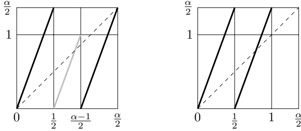
Figure 4.2. The map T_\sigma
