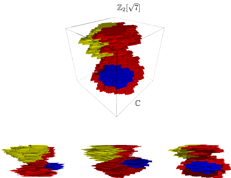
Figure 10.9. Pictures of the central tile \mathcal{R}_\sigma divided in the red (gray) subtile \mathcal{R}_\sigma(1) , the blue (dark gray) \mathcal{R}_\sigma(2) and the yellow (light gray) \mathcal{R}_\sigma(3) .
