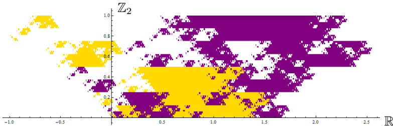
Figure 4.3. The central tile \mathcal{R}_\sigma for \sigma(1) = 2121^3 , \sigma(2) = 12 subdivided in the purple (dark gray) subtile \mathcal{R}_\sigma(1) and the yellow (light gray) subtile \mathcal{R}_\sigma(2) . (1) Here we represented each \sum_{i=0}^\infty d_i \alpha^i \in \mathbb{Z}_2 by \sum_{i=0}^\infty d_i 2^{-i-1} \in [0, 1] , with d_i \in \{0, 1\} .
