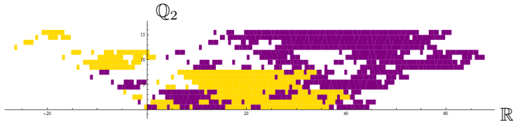
Figure 4.5. T_{\text{ext}}^{-4}((\mathbf{0}, 1) \cup (\mathbf{0}, 2)) projected into K_{\sigma} .
