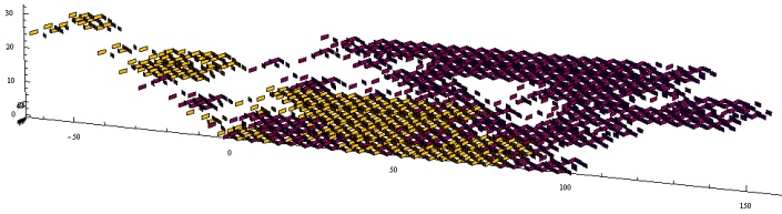
Figure 1.2. T_{\text{ext}}^{-5}(\mathcal{U}) for the substitution \sigma(1) = 2121^3 , \sigma(2) = 12 .
