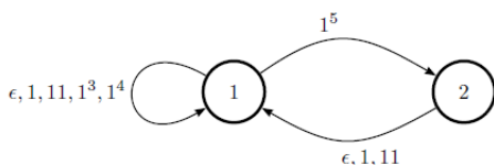
Figure 10.1. Prefix automaton of \sigma .
