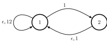
Figure 4.1. The prefix automaton of the substitution \sigma(1) = 121 , \sigma(2) = 11 .
