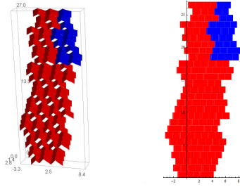
Figure 10.6. T_{\text{ext}}^{-3}(\mathcal{U}) and its projection into K_\sigma .
