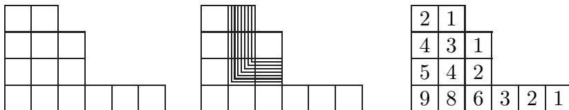
Figure 1.1. Partition. Figure 1.2. Hook length. Figure 1.3. Hook lengths.
