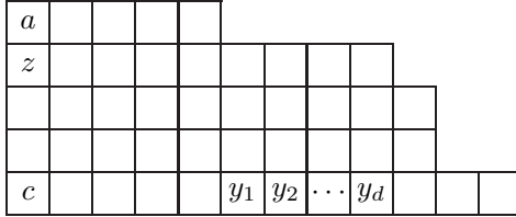
Figure 2.1. Hook length and t -compact set.
