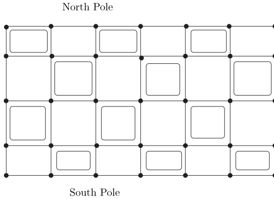
Figure 2.2. A perturbation in degree 2m = 6 . The black dot \bullet denotes positive sign of Y_6^6 at singular points of Y_6^3 . Note that on S^2 all points on the top line (north pole) and the bottom line (south pole) are identified.
