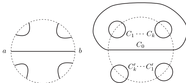
Figure 1.1. A chord diagram producing ovals
