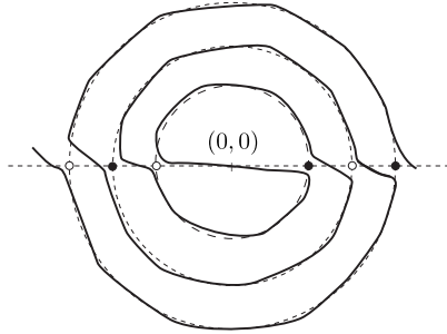
Figure 3.1. A function in \mathbb{R}^2 with two nodal domains. Dashed line denotes the nodal set of f = J_1(r) \sin \theta , solid line denotes the nodal set of the perturbed eigenfunction h . The black dot \bullet denotes positive sign of g at singular points of f , the white dot \circ denotes negative sign of g at singular points of f .
