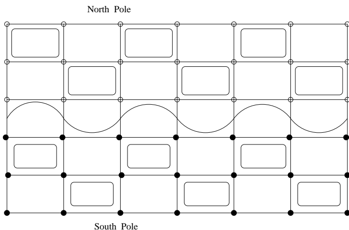
Figure 2.1. A perturbation in degree 4k + 3 = 7 . The black dot \bullet denotes positive sign of Y_7^6 at singular points of Y_7^3 , while the white dot \circ denotes negative sign of Y_7^6 at singular points of Y_7^3 . Note that on S^2 all points on the top line (north pole) and the bottom line (south pole) are identified.
