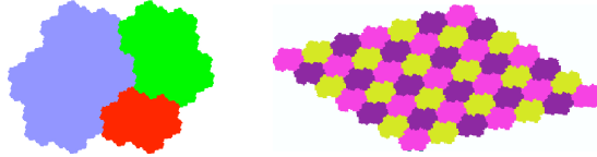
Figure 4.3. Rauzy fractal for the Tribonacci substitution, and Rauzy lattice tiling
