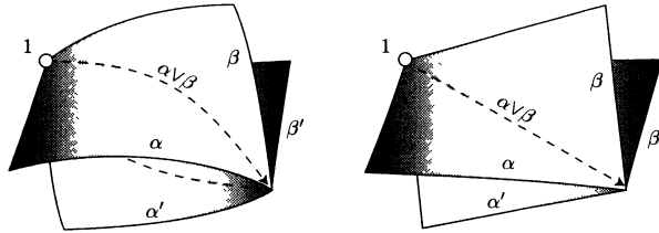
Figure 13. Going from \mathcal{T} to \mathcal{T}' by pinching common edges
