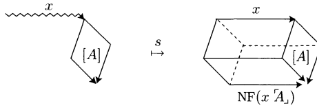
Figure 9. The contracting homotopy s
