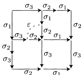
Figure 1. Word reversing diagram for the standard presentation of B_4^+
