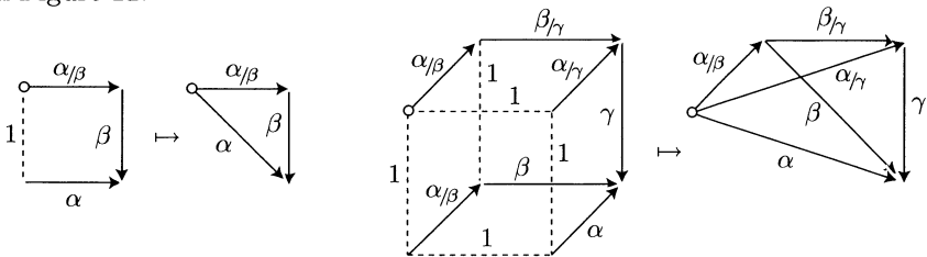
Figure 11. The n -simplex associated with a descending n -cell
