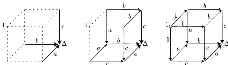
Figure 3. The 3-cube associated with a 3-cell, case of BKL_3^+
