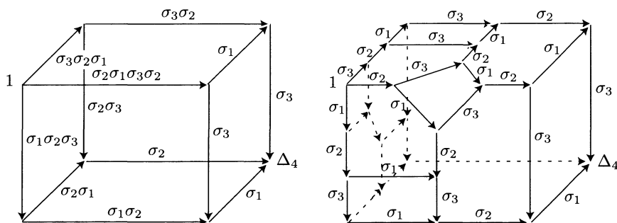
Figure 4. The 3-cube associated with the 3-cell [\sigma_1, \sigma_2, \sigma_3] in B_4^+ when the generators are the divisors of \Delta_4 (left) and when they are the \sigma_i 's (right)
