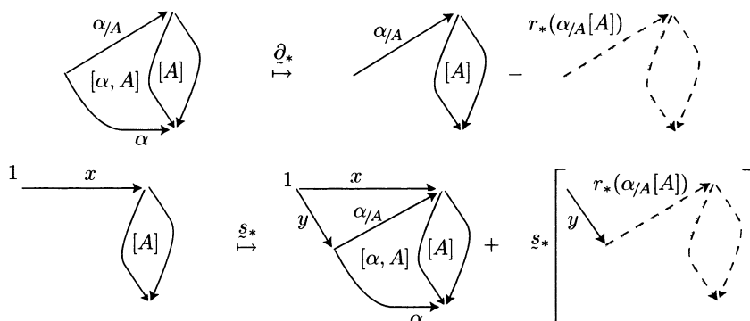
Figure 14. The boundary operator \partial_* and the section \underline{s}_*
