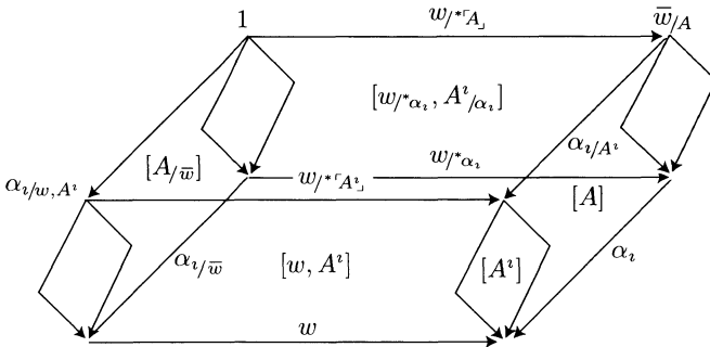
Figure 7. Decomposition of [w, A]
