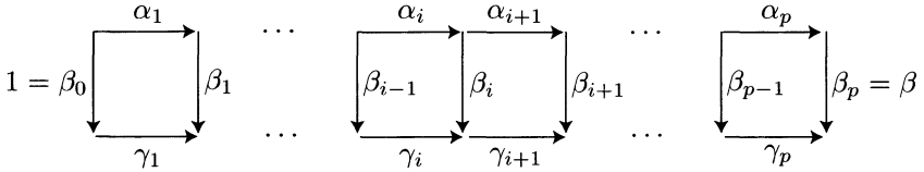
Figure 2. Computing the normal form using reversing
