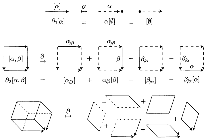
Figure 5. The boundary operator \partial
