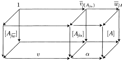
Figure 6. The chain [w, A] for w = v\alpha
