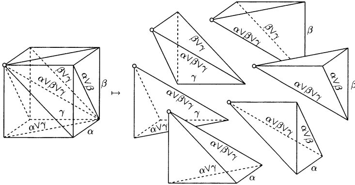
Figure 12. Decomposition of a cube into six tetrahedra
