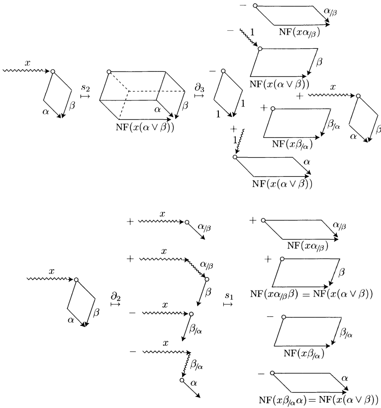
Figure 10. Comparing \partial_3 s_2(x[\alpha, \beta]) and s_1 \partial_2(x[\alpha, \beta]) : in the sum, there remain only the trivial left face, and x[\alpha, \beta] itself.
