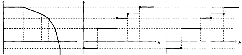
Symmetric of the Newton polygon of D
