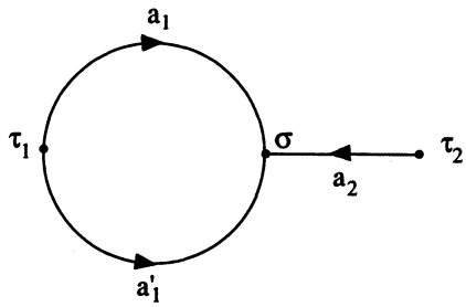
Its opposite C^{op}
