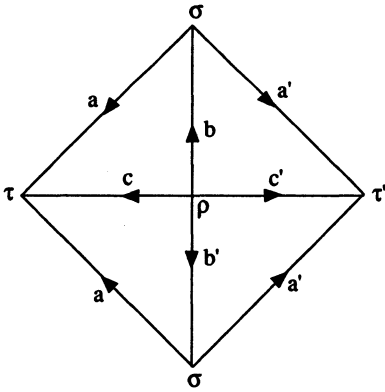
Ordered simplicial cell complex X homeomorphic to S^2 (elements with the same label should be identified)
