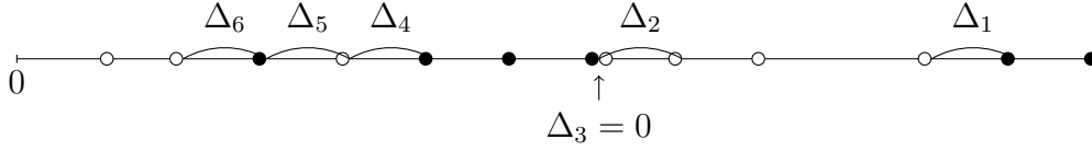
Figure 4.1. A sequence of gaps, as defined in (4.100). The white and black dots are the points in I and J , respectively.
