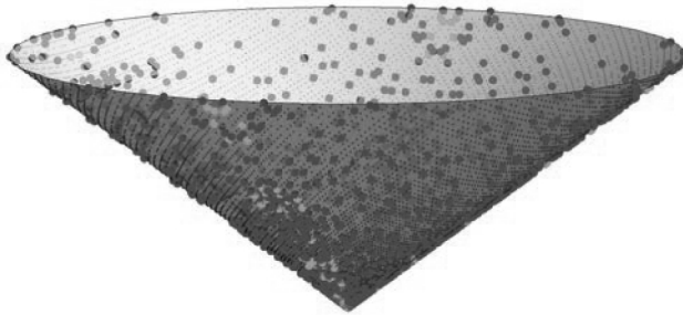
Figure 1. — A piece of the cone V in (3.9) with markings at the primitive Pythagorean triples \mathbf{x} . Points \mathbf{x} are marked according to whether the “area” f(\mathbf{x}) = \frac{1}{12}xy is in \mathcal{P}_R with R \leq 3 (●), R = 4 (●), or R \geq 5 (●).
