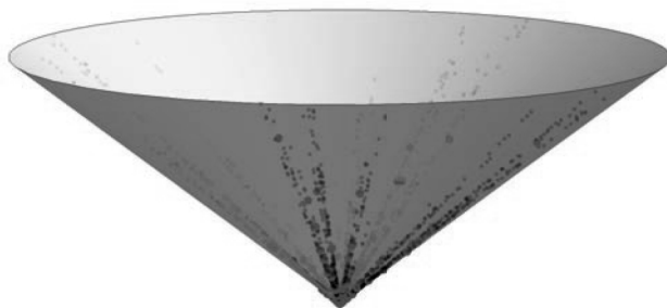
Figure 2. — A piece of the thin Pythagorean orbit \mathcal{O} in (3.28). Points \mathbf{x} \in \mathcal{O} are again marked according to whether the “area” f(\mathbf{x}) = \frac{1}{12}xy is in \mathcal{P}_R with R \leq 3 (●), R = 4 (●), or R \geq 5 (●).
