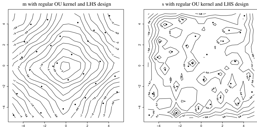
Figure 5. — Simple Kriging mean and standard deviation with the regular tensor product kernel of Eq. 4.9, based on observations of y at \mathbf{X} .
