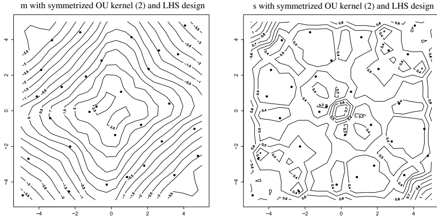
Figure 8. — Kriging mean and standard deviation with the symmetrized OU kernel of Eq. 4.12, based on observations of y at \mathbf{X} .
