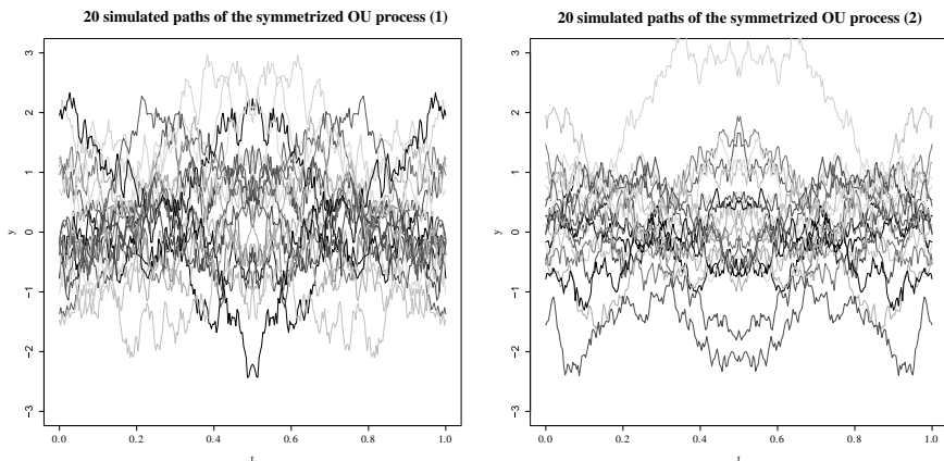
Figure 2. — Symmetrization of the OU process relying on both kernels defined by Eqs. 4.6, 4.8. Left: by projection on a fundamental domain (Eq. 4.6). Right: by averaging over the orbits (Eq. 4.8).
