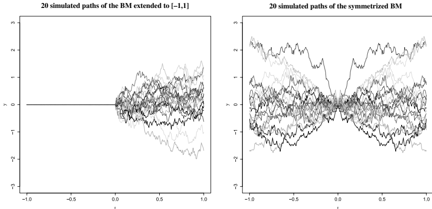
Figure 1. — Symmetrization of the Brownian Motion relying on the symmetrized kernel (by projection on a fundamental domain) of Eq. 4.2.
