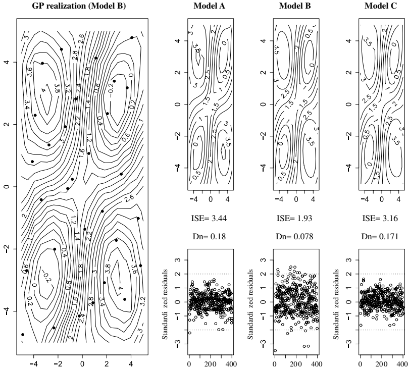
Figure 12. — Left: Simulation of a Gaussian Field with argumentwise invariant kernel (Model B), and learning set \mathbf{X} (black points). Right, for each of the three columns: Kriging mean (above) and standardized residuals when predicting at \mathbf{X}_{\text{val}} with Kriging models A, B, and C. The ISE values quantify the departure of the Kriging mean from the actual function. The D_n values (Kolmogorov’s statistic) quantify the departure from normality of the standardized residuals.
