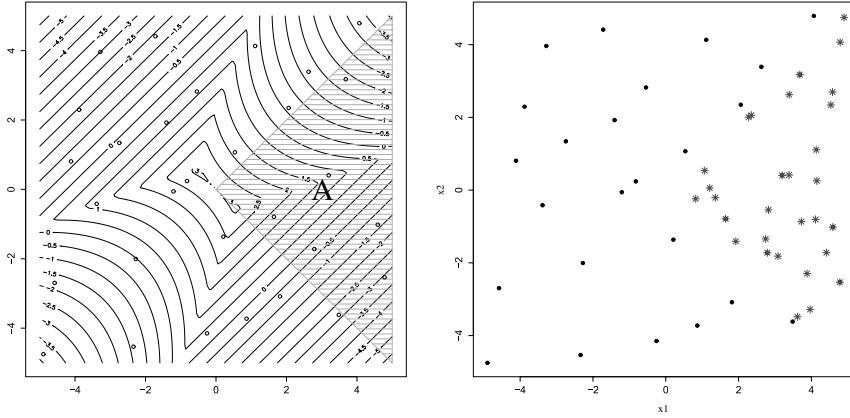
Figure 6. — Left: The fundamental domain A for the considered action of (\mathbb{Z}/2\mathbb{Z})^2 on [-5, 5]^2 . The lower left boundary is excluded. Right: Projection of the design points of \mathbf{X} (black points) onto A (red stars).
