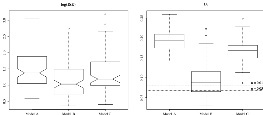
Figure 13. — Left: log-ISE values (at \mathbf{X}_{\text{val}} ) when using the three Kriging models A, B, C for predicting 100 Gaussian Field realizations generated with Model B .
