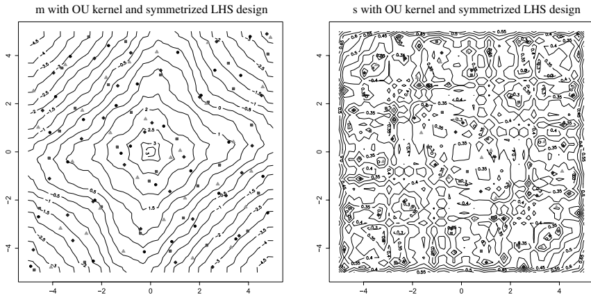
Figure 9. — Kriging mean and standard deviation with the regular tensor product kernel of Eq. 4.9, based on observations of y at \mathbf{X}_{\text{sym}} . The solid black circles represent the LHS design \mathbf{X} . The red squares, blue diamonds, and green triangles represent respectively the orbits of \mathbf{X} under the transformations s_1, s_2 , and s_3 .
