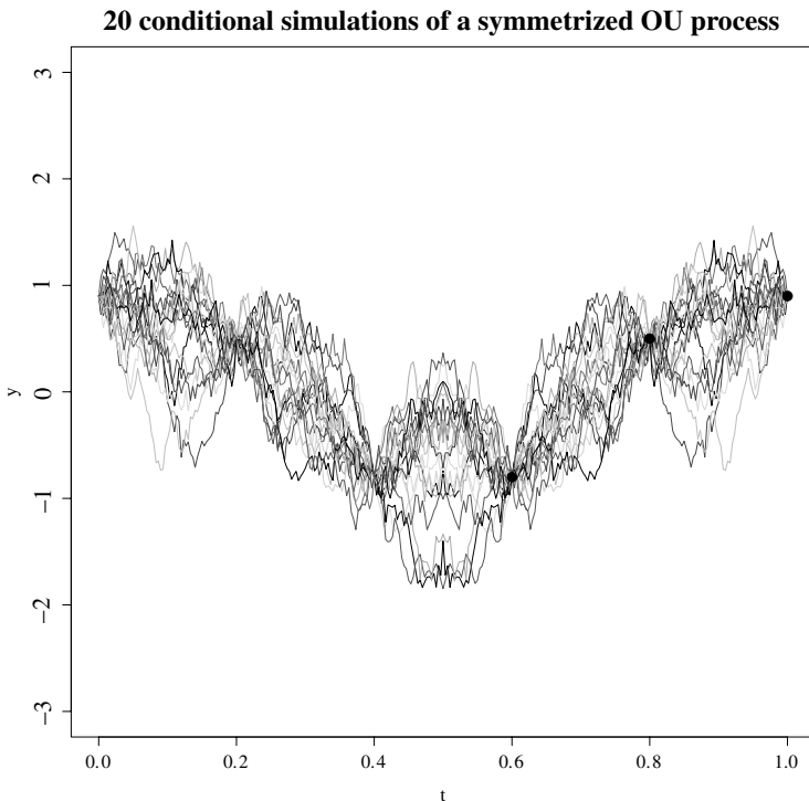
Figure 3. — Conditional Simulations of the symmetrized OU process with the kernel of Eq. 4.8. The black points stand for the conditioning data.
