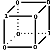
Figure 3. — Kronecker (2 \times 2 \times 2) tensor.
