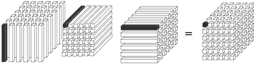
Figure 1. — Tensor's ternary Product.
