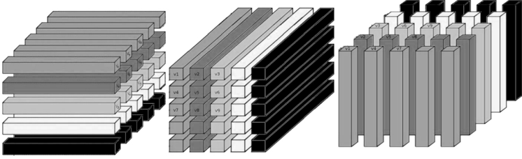
Figure 5. — Orthogonal slices of an orthogonal tensor.
