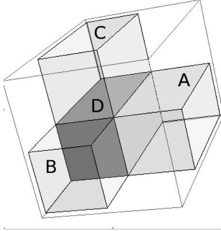
Figure 2. — Constraints on the dimensions of the tensors implied by the ternary product definition.
