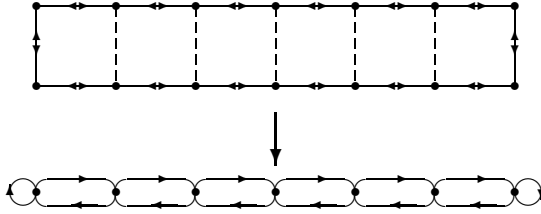
Figure 2. — The 2n cycle collapses to the n -stick with loops at the ends, n = 7 . All edges have weight 1/2 .
