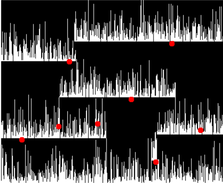
FIGURE 11. Simulation with \beta = \infty .
