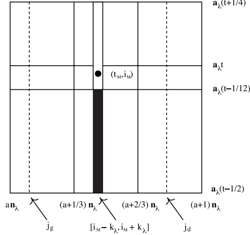
FIGURE 7. The event \Omega_{a,t}^\lambda .
