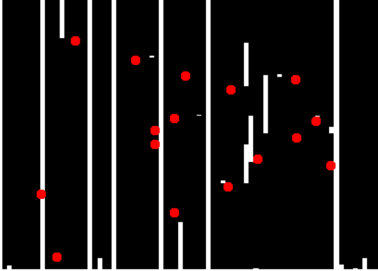
FIGURE 14. Simulation with \beta = 0 .
