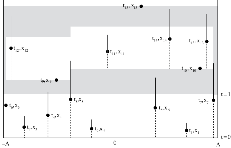
FIGURE 2. LFF( \infty )-process in a finite box.
