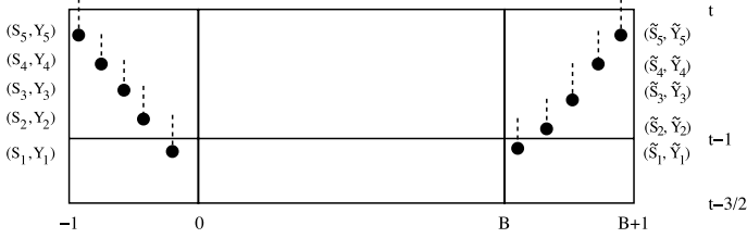
FIGURE 9. The event \Omega_{t,B} .
