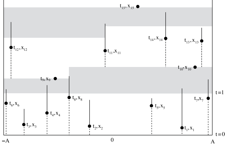
FIGURE 3. LFF(BS)-process in a finite box.
