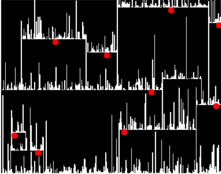
FIGURE 13. Simulation with \beta = 2 .
