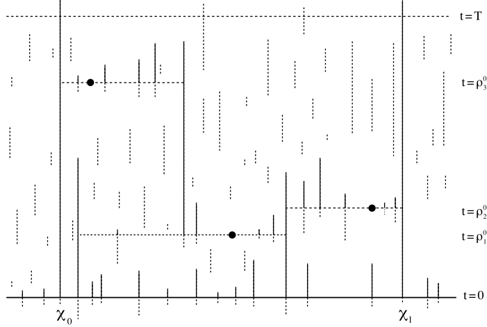
FIGURE 4. LFF( \beta )-process with \beta \in (0, \infty) .
