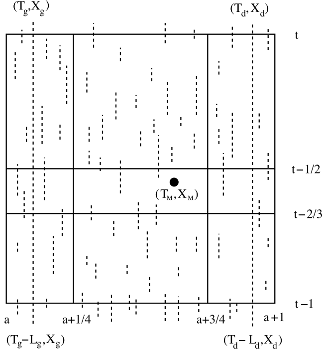
FIGURE 6. The event \Omega_{t,A} .
