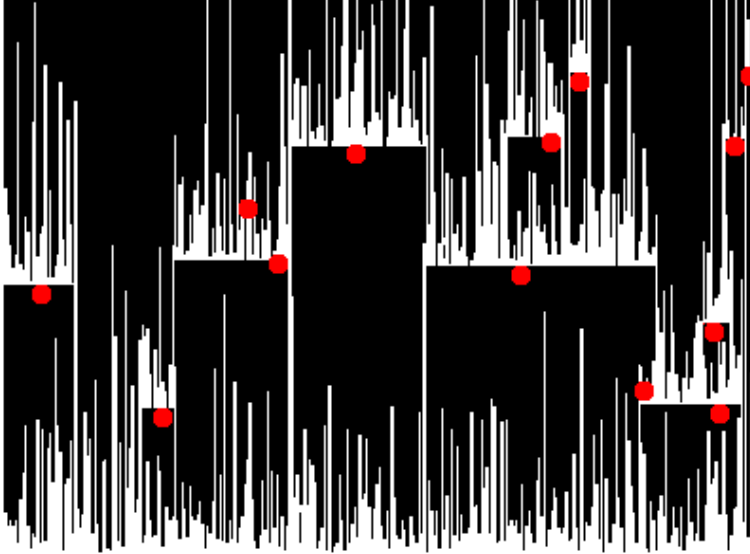
FIGURE 12. Simulation with \beta = 5 .
