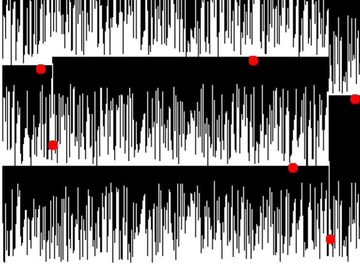
FIGURE 10. Simulation with \beta = BS .
