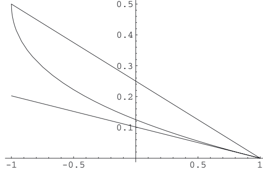
FIGURE 7. 0.2023\frac{1-x}{2} versus \frac{1}{2}\frac{1-x}{2} versus (\arccos(x)/\pi)^2\frac{1}{2} .
