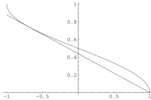
FIGURE 6. \frac{\arccos(x)}{\pi} versus 0.878 \left(\frac{1-x}{2}\right) .
