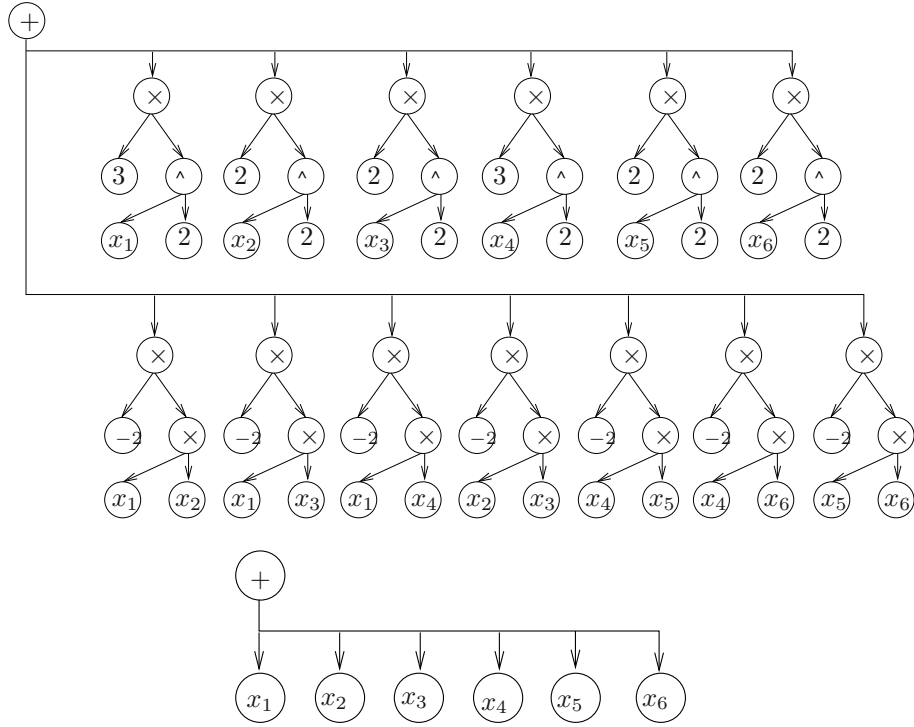
FIGURE 1. The graphs e_1 (top) and e_2 (bottom) from Example 3.2.
