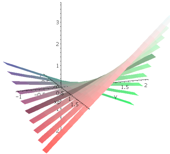
FIGURE 5. Linearizing approximation of a bilinear term.
