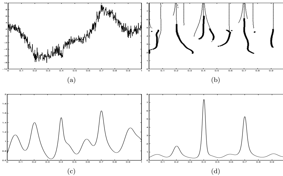
FIGURE 2. (a) Noisy signal f_3 with RSNR = 5, n = 512 . (b) Estimated wavelet maxima (thick lines) and true wavelet maxima (thin lines) for r = 2 . (c) Non-weighted structural intensity of the estimated wavelet maxima. (d) Weighted structural intensity of the estimated wavelet maxima.
