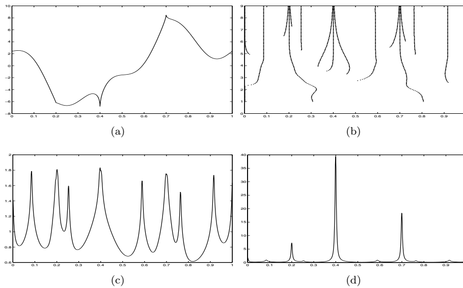
FIGURE 1. (a) Signal f_3 (see expression (2.3)). (b) Wavelet maxima of f_3 computed with a B-Spline of order 4 with r = 2 vanishing moments. (c) Non-weighted structural intensity of the wavelet maxima (d) Weighted structural intensity of the wavelet maxima.
