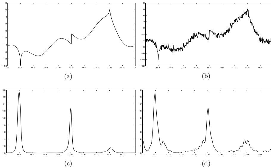
FIGURE 4. (a) Signal f_T (see expression (4.2)). (b) Noisy signal f_T with RSNR = 7, n = 512 . (c) EstWMSt: structural intensity of the estimated wavelet maxima for r = 3 . (d) DenSt: structural intensity of the wavelet maxima of \hat{f}_T (obtained by SureShrink thresholding) for r = 3 .
