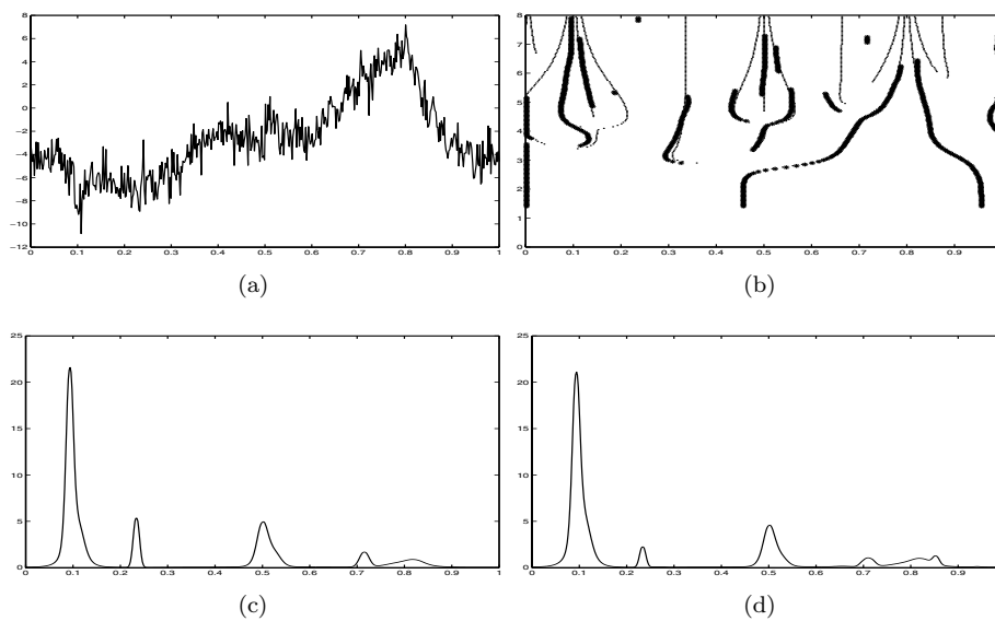
FIGURE 6. An example of bagging for removing spurious estimates: (a) Noisy signal f_T with RSNR = 3 , n = 512 . (b) Estimated wavelet maxima (thick lines) and true wavelet maxima (thin lines) for r = 3 : note the presence of some spurious wavelet maxima at fine scales. (c) Weighted structural intensity of the estimated wavelet maxima. (d) Weighted structural intensity \hat{G}_m^{(Bag)}(x) of the estimated wavelet maxima after bagging.
