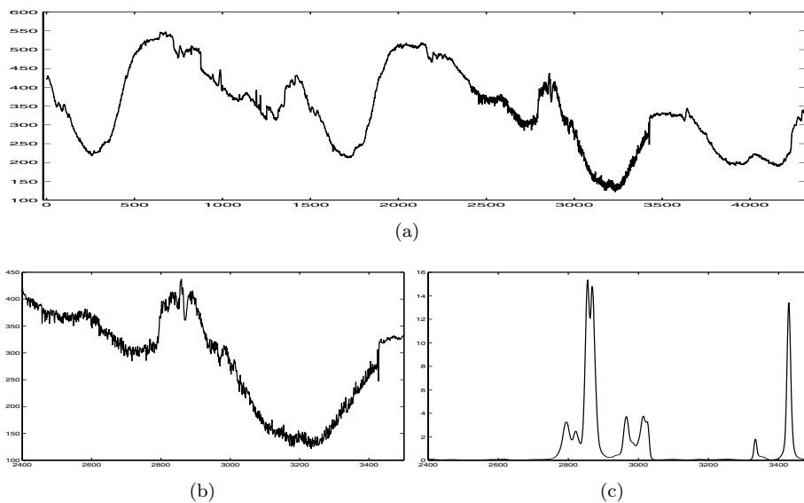
FIGURE 7. (a) An electrical consumption signal over the course of 3 days. (b) Signal e(t) . (c) Average structural intensity G(t) .
