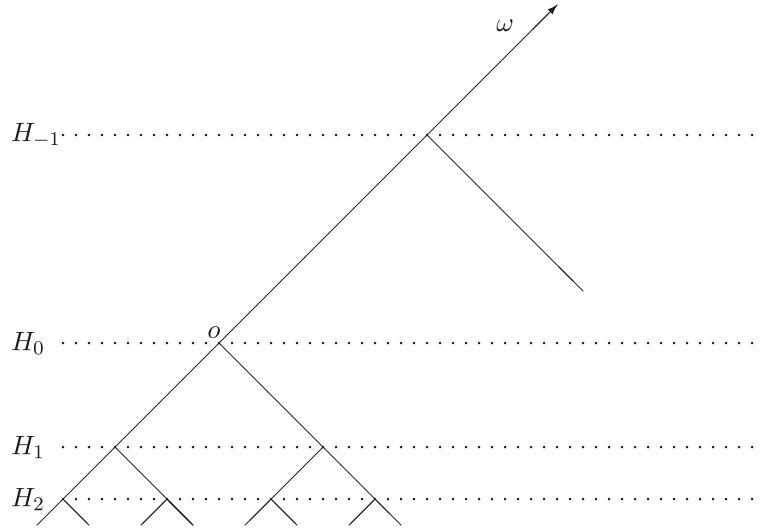
FIGURE 5. A part of the tree rooted at \omega and horocycles corresponding to o .
