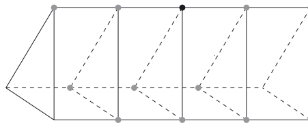
FIGURE 3. Set of local configurations of a spider with bounded span ( k = s = 2 ) on the direct product \mathbb{Z}_3 \times \mathbb{Z} .
