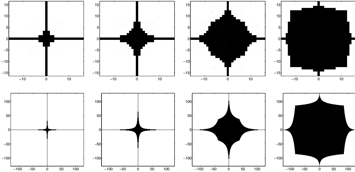
FIGURE 2. Index sets \hat{\Omega}_{16,T} (above) and \hat{\Omega}_{128,T} (below) for T = 0.5, 0, -2, -10 (from left to right), d = 1, N = 2 ; the hyperbolic cross corresponds to T = 0 .
