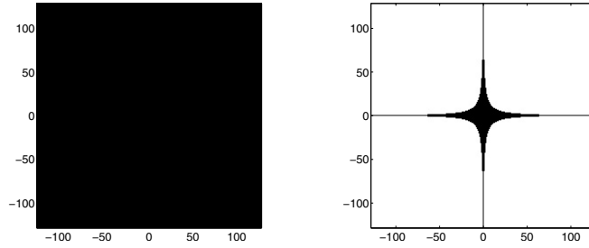
FIGURE 1. The (full) grid \hat{\Omega}_{K,-\infty} (left) and the sparse grid \hat{\Omega}_{K,0} , for d = 1 , N = 2 and K = 128 .
