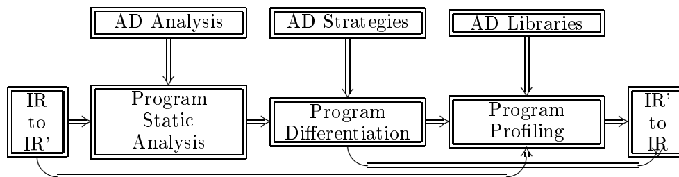
FIGURE 2. AD kernel.
