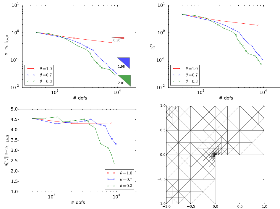
FIGURE 4. Error, estimator, effectivity index, and adaptively generated mesh ( k = 5 ).
