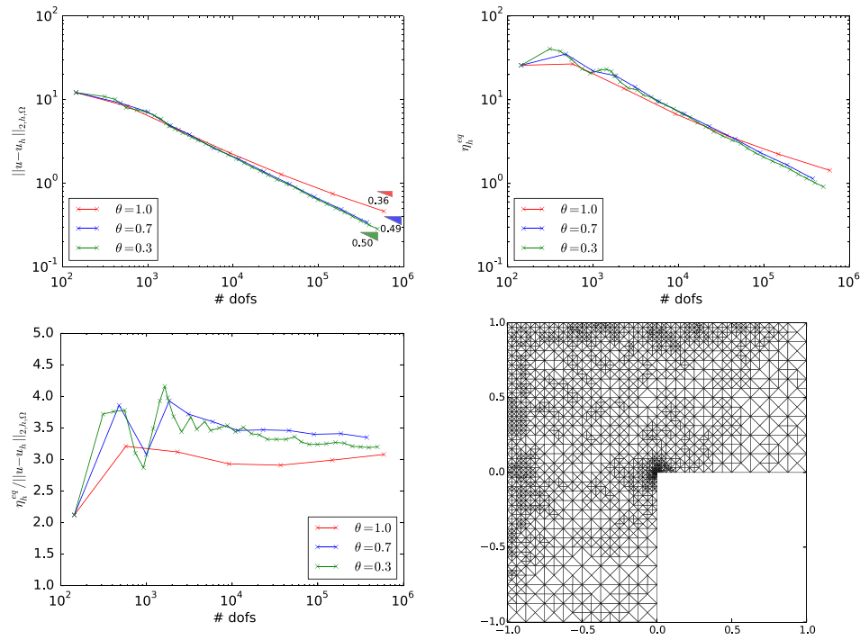
FIGURE 1. Error, estimator, effectivity index, and adaptively generated mesh ( k = 2 ).
