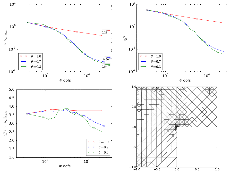
FIGURE 3. Error, estimator, effectivity index, and adaptively generated mesh ( k = 4 ).
