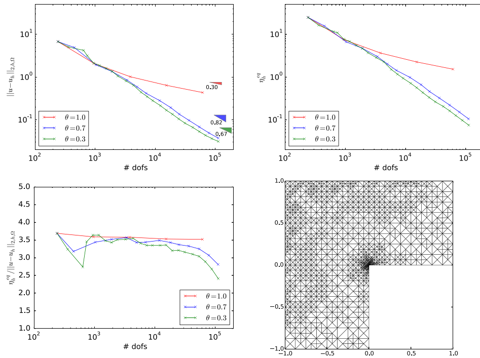
FIGURE 2. Error, estimator, effectivity index, and adaptively generated mesh ( k = 3 ).
